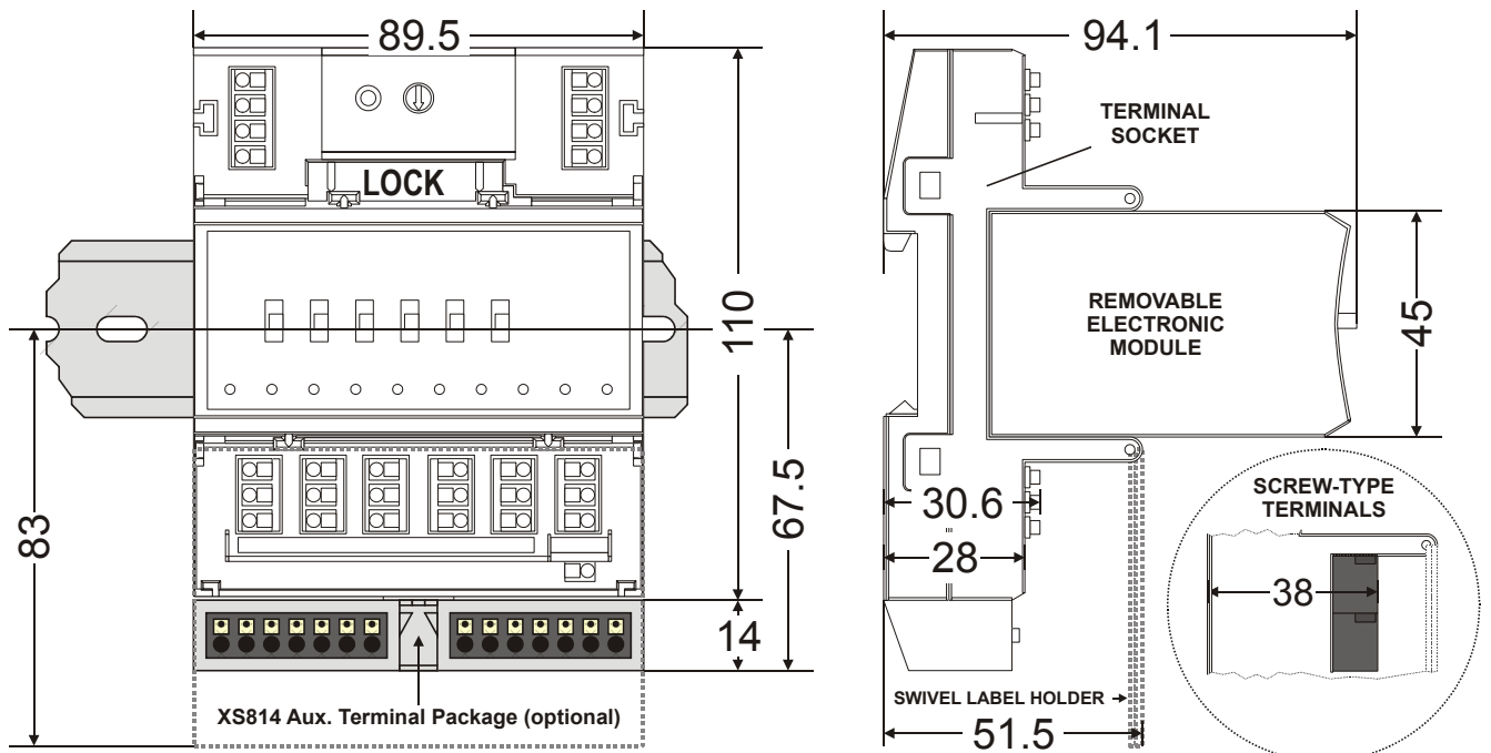
Fig. 25. Pluggable Excel 800 I/O Modules (example shows Manual Overrides), incl. Terminal Socket, dimensions (in mm)
