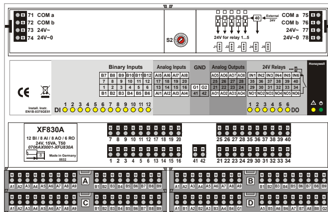
Fig. 22. XF830A mixed Excel 800 Panel Bus I/O module, shown with 4 optional aux. terminal blocks (top view)
