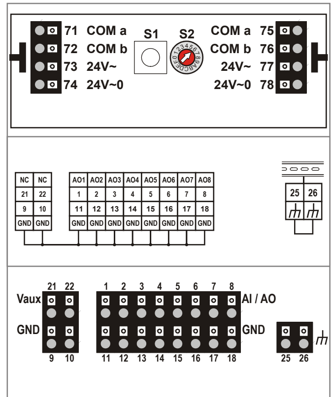
Fig. 13. Excel 800 Analog Output Modules (schematic)
