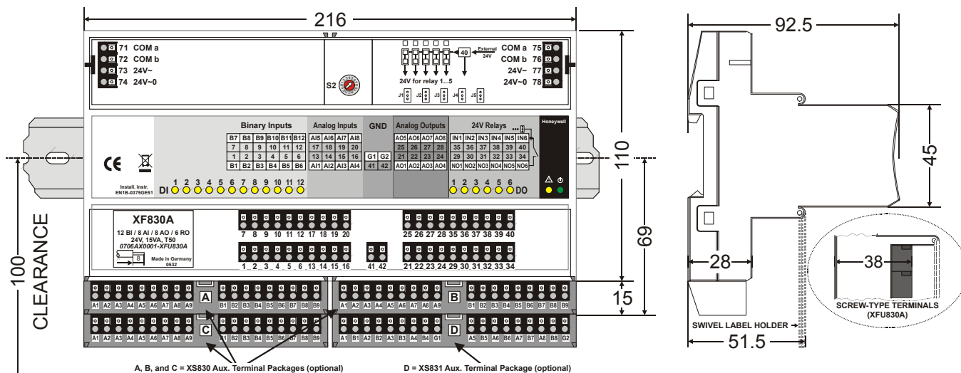
Fig. 26. Mixed Excel 800 I/O Modules (example shows XF830A with 4 auxiliary terminal packages), dimensions (in mm)
