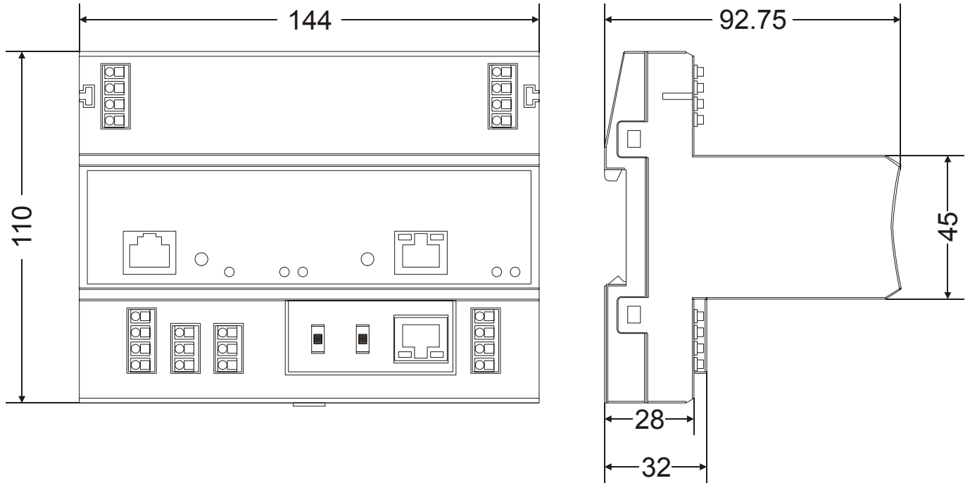
Fig. 24. XCL8010A Controller Module, dimensions (in mm)
