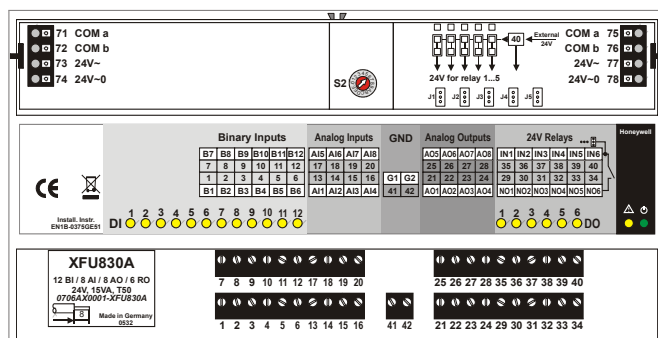
Fig. 23. XFU830A mixed Excel 800 Panel Bus I/O module, shown without optional aux. terminal blocks (top view)
