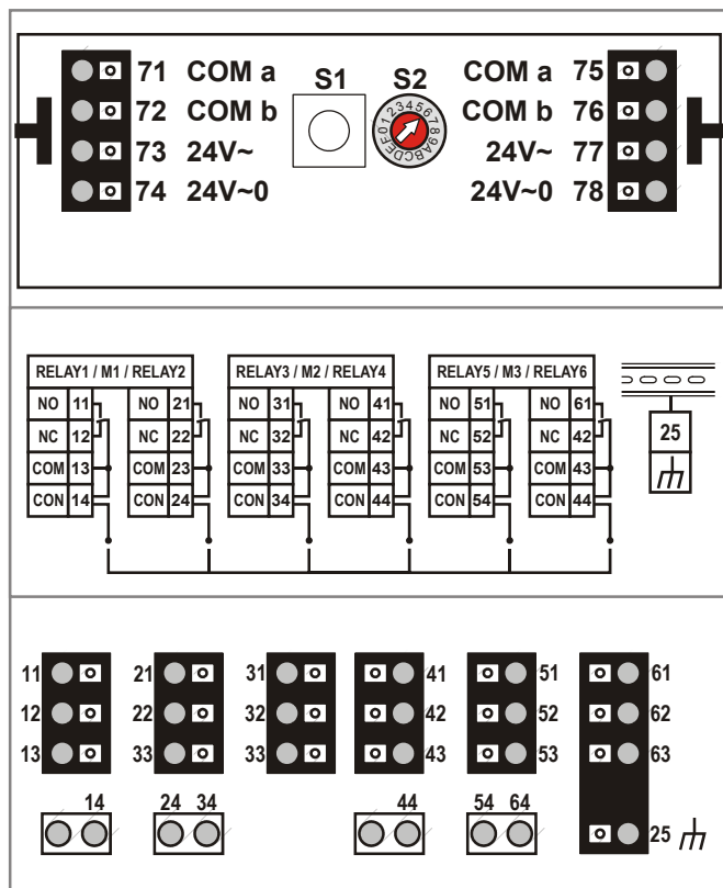
Fig. 20. XFR825A Panel Bus Floating Output Module (schematic)
