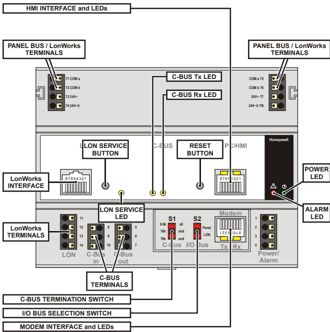
Fig. 4. XCL8010 Controller Module features
