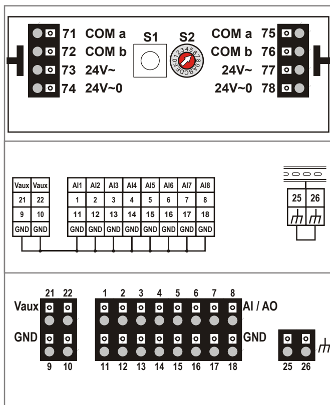
Fig. 10. Excel 800 Analog Input Modules (schematic)
