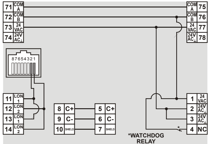
Fig. 5. XCL8010A Controller Module, terminal assignment
