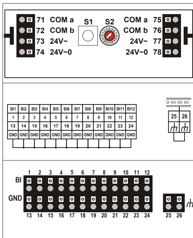
Fig. 15. Excel 800 Binary Input Modules (schematic)
