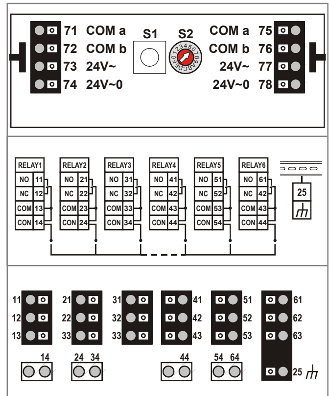
Fig. 18. Excel 800 Relay Output Modules (schematic)
